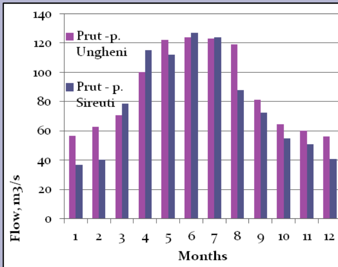
Figure 2. The monthly distribution of average flow (m 3 / s)
