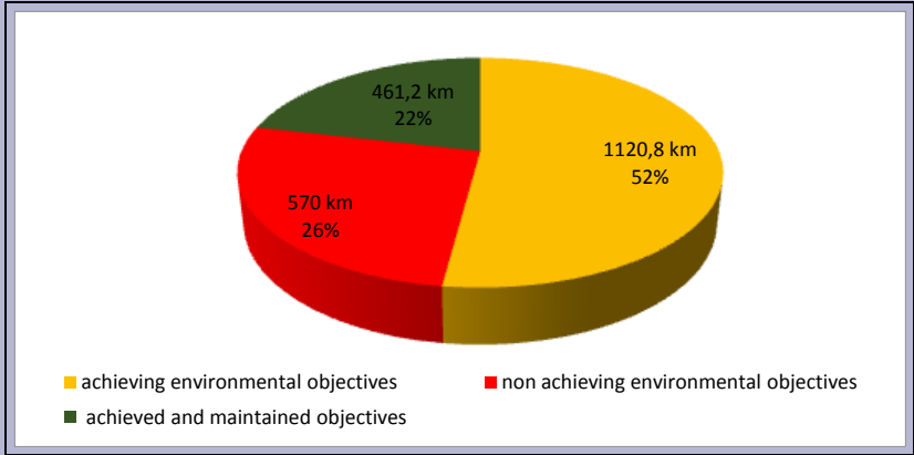
Figure 21. Achieving and maintaining environmental objectives in the second cycle (until 2027)
