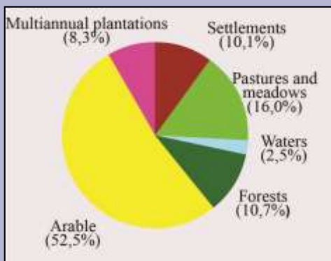
Figure 4. Land use in the Prut River Basin
