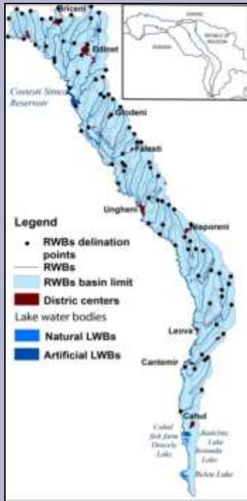
Figure 6. Surface water bodies in the Prut River basin of Moldova
