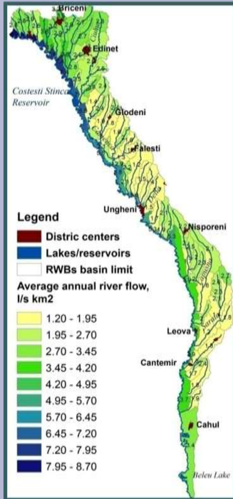
Figure 3. The spatial variation of average effective flow of the Prut River
