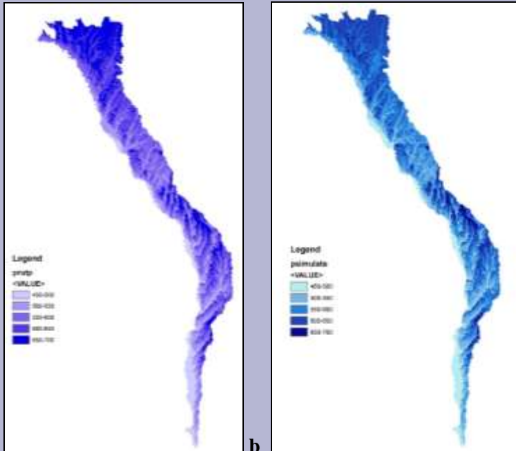
Figure 25. Spatial distribution of annual amount of precipitation in the period 1986-2005 (a) and the simulated model for the years 2016-2035 according to RCP4.5 (b)
