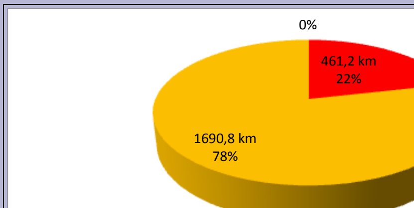
Figure 20. Achieving environmental objectives in the first cycle (until 2022)
