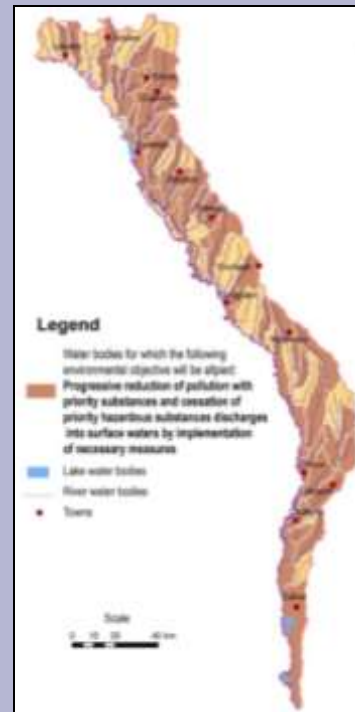
Figure 17. Water bodies for application of the environmental objective „Progressive reduction of pollution”
