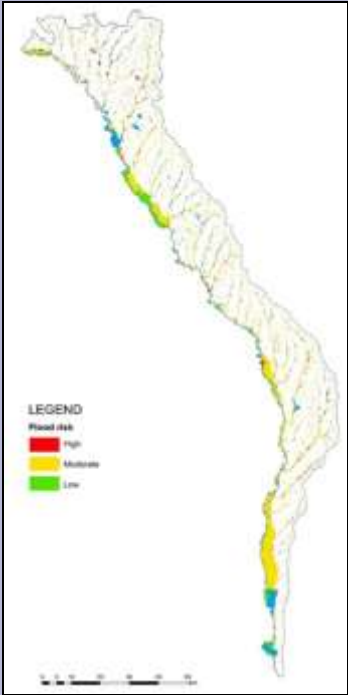
Figure 26. Susceptibility to flooding
