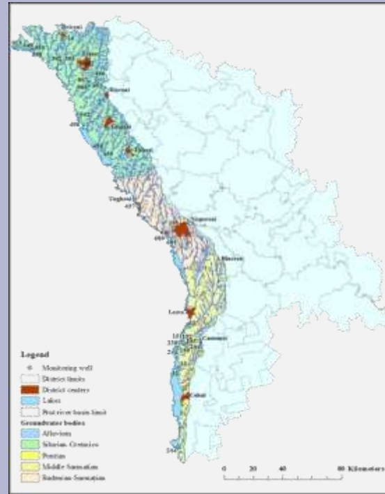
Figure 7. Groundwater bodies and monitoring wells in the limits of the Prut River Basin
